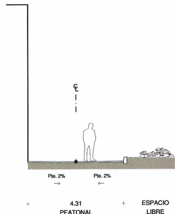
PEATONAL "I" 4.31 m.
